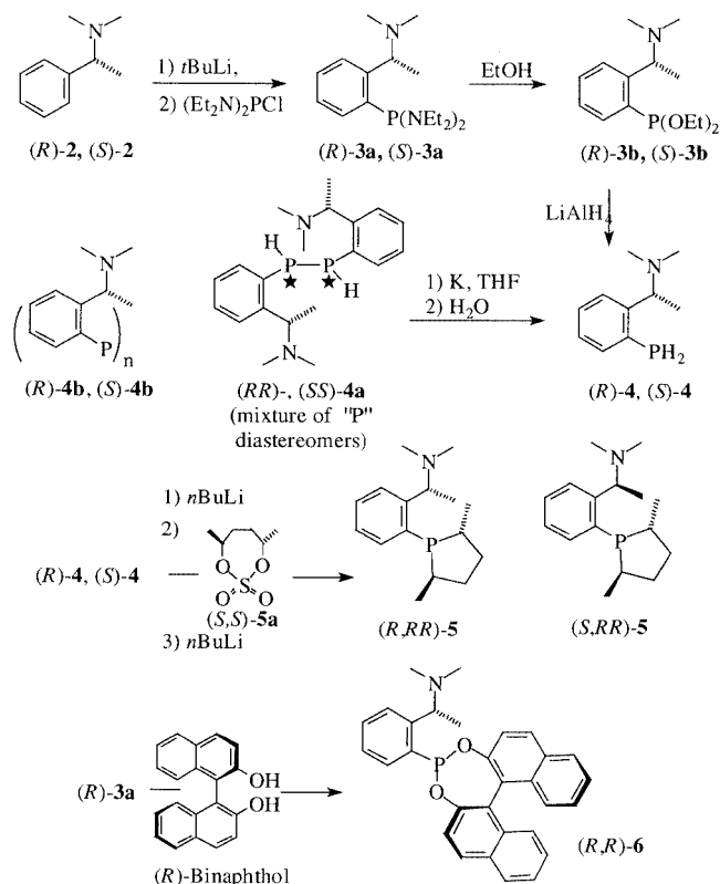
Scheme 1. Syntheses of the chiral P,N ligands
