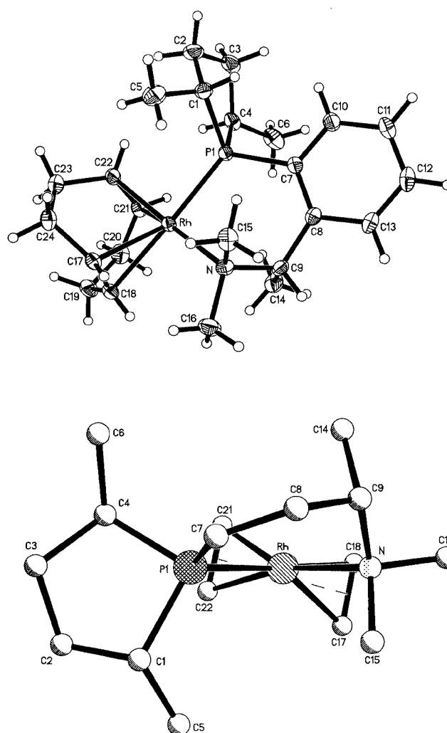
Figure 2. Structure of the cation of ( S,RR )- 7a (top); front view, showing the orientation of the phospholane group and the chelate ring of ( S,RR )- 7a (bottom); hydrogen atoms have been omitted for clarity
