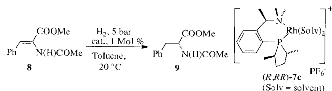
Scheme 3. Hydrogenation of methyl ( Z )- \alpha -acetamidocinnamate
