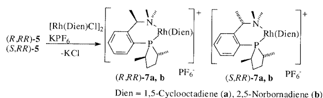
Scheme 2. Syntheses of the complexes ( R,RR )- 7a , ( R,RR )- 7b , ( S,RR )- 7a , and ( S,RR )- 7b
