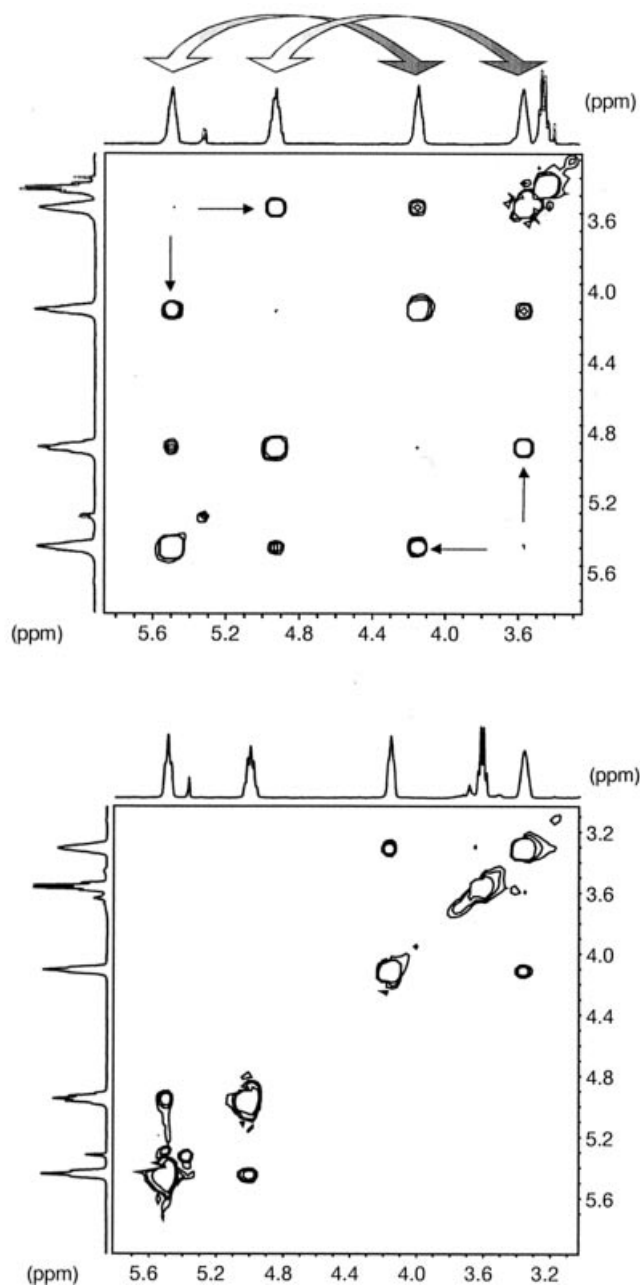
Figure 3. 400 MHz ^1\text{H} -NOESY spectra at 300 K in \text{CD}_2\text{Cl}_2 of ( R,RR )- 7a (top) and ( S,RR )- 7a (bottom); signals caused by chemical exchange are indicated with arrows; a mixing time of 1.0 s was used
