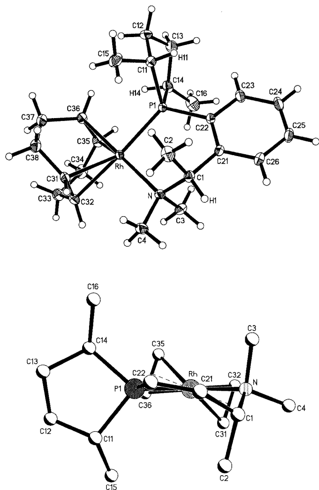
Figure 1. Structure of the cation of ( R,RR )- 7a (top); front view, showing the orientation of the phospholane group and the chelate ring of ( R,RR )- 7a (bottom); hydrogen atoms have been omitted for clarity
